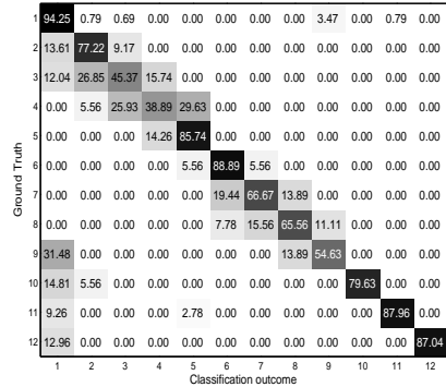
(b) SVM with Poly5 and DTW metric.
