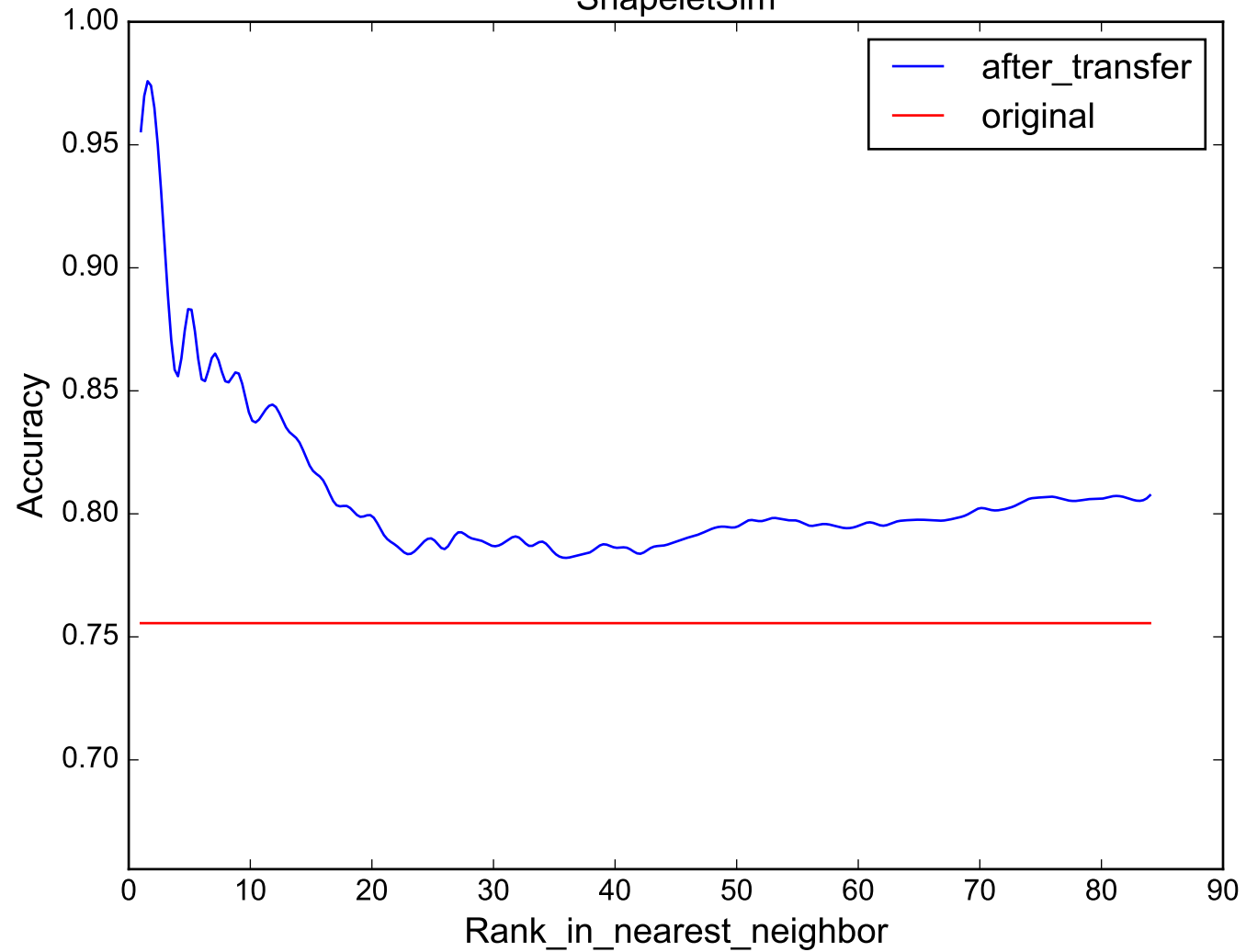
ShapeletSim
