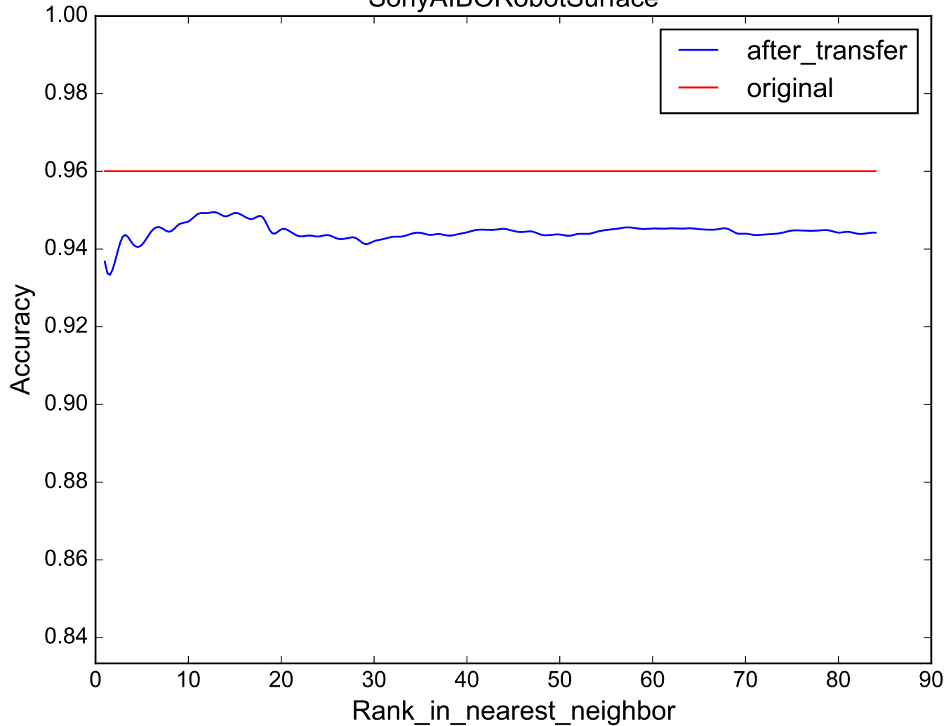
SonyAIBORobotSurface
