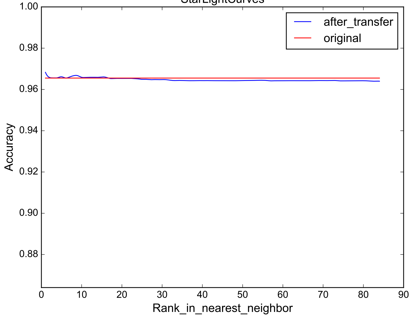
StarLightCurves
