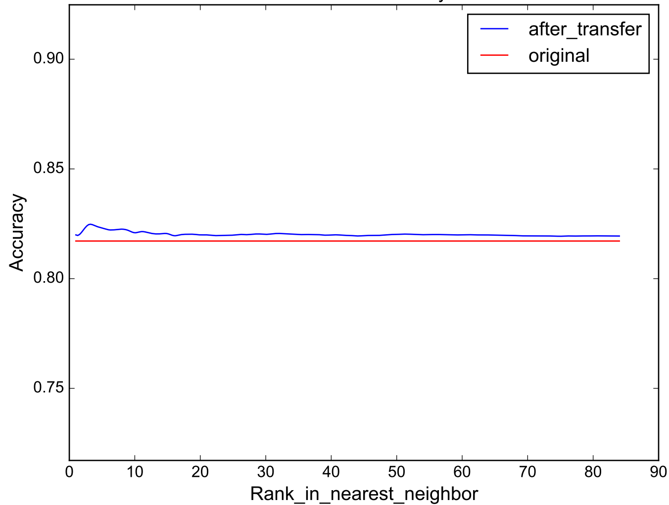
UWaveGestureLibraryAll
