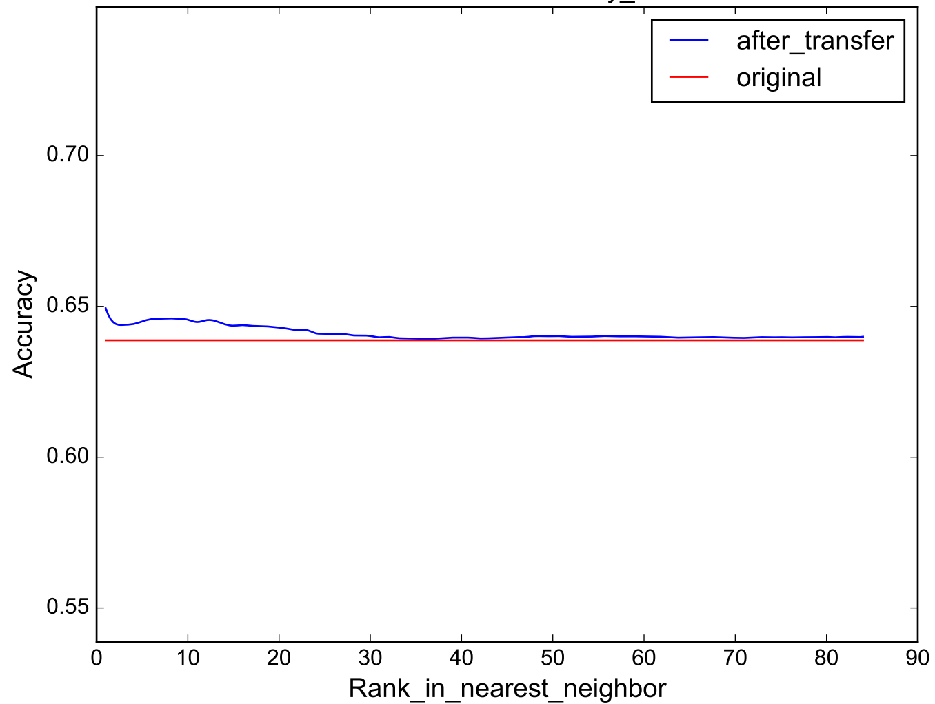
uWaveGestureLibrary_Y
