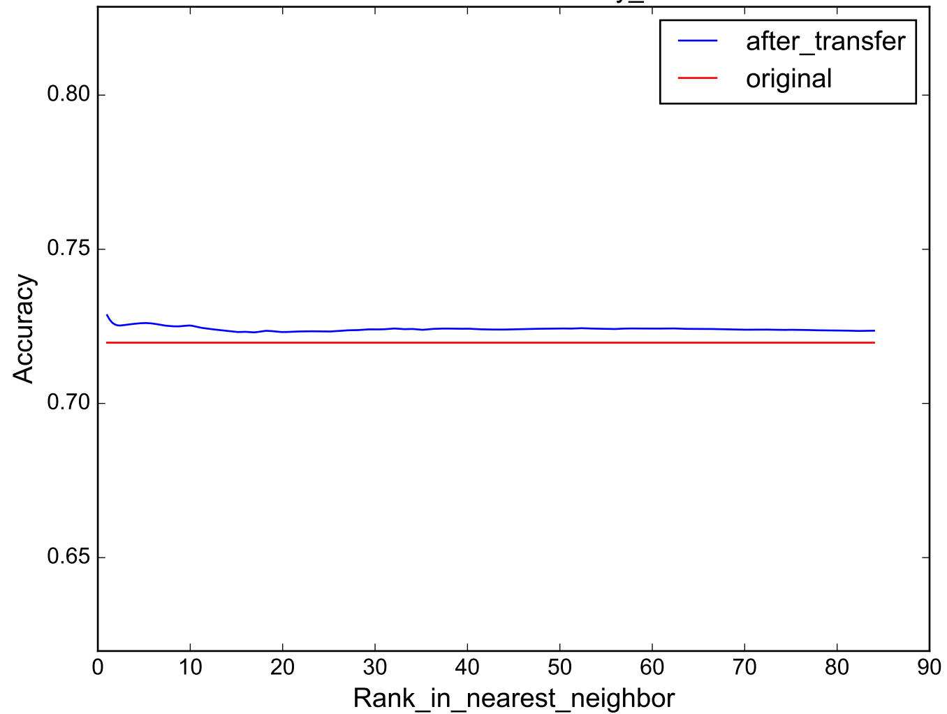
uWaveGestureLibrary_Z
