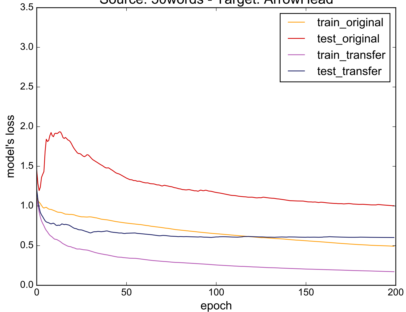
Source: 50words - Target: ArrowHead
