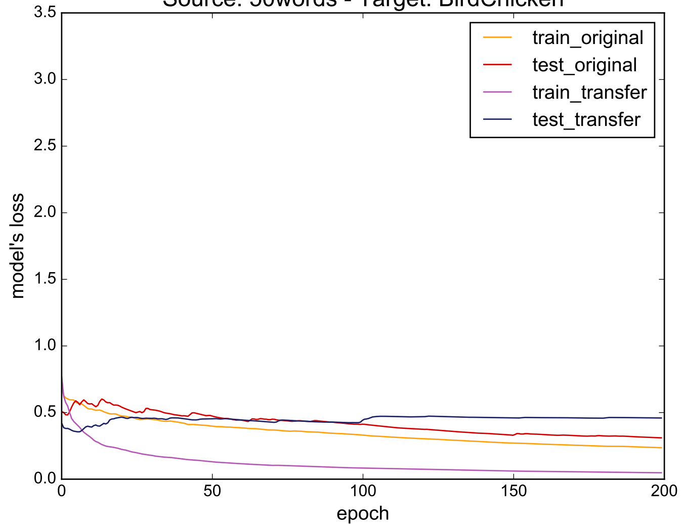
Source: 50words - Target: BirdChicken
