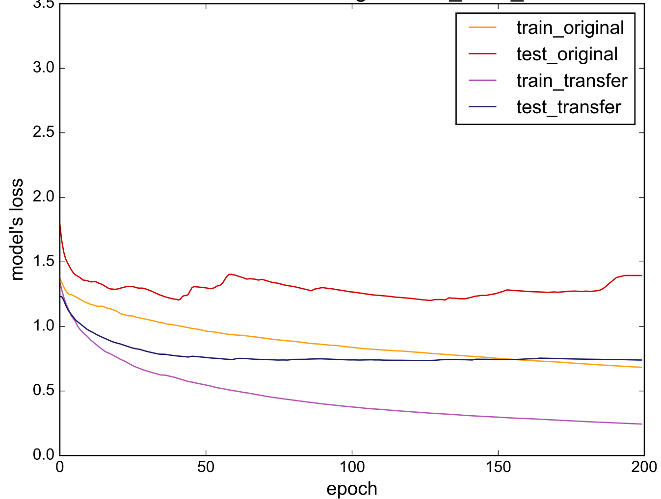
Source: 50words - Target: CinC_ECG_torso
