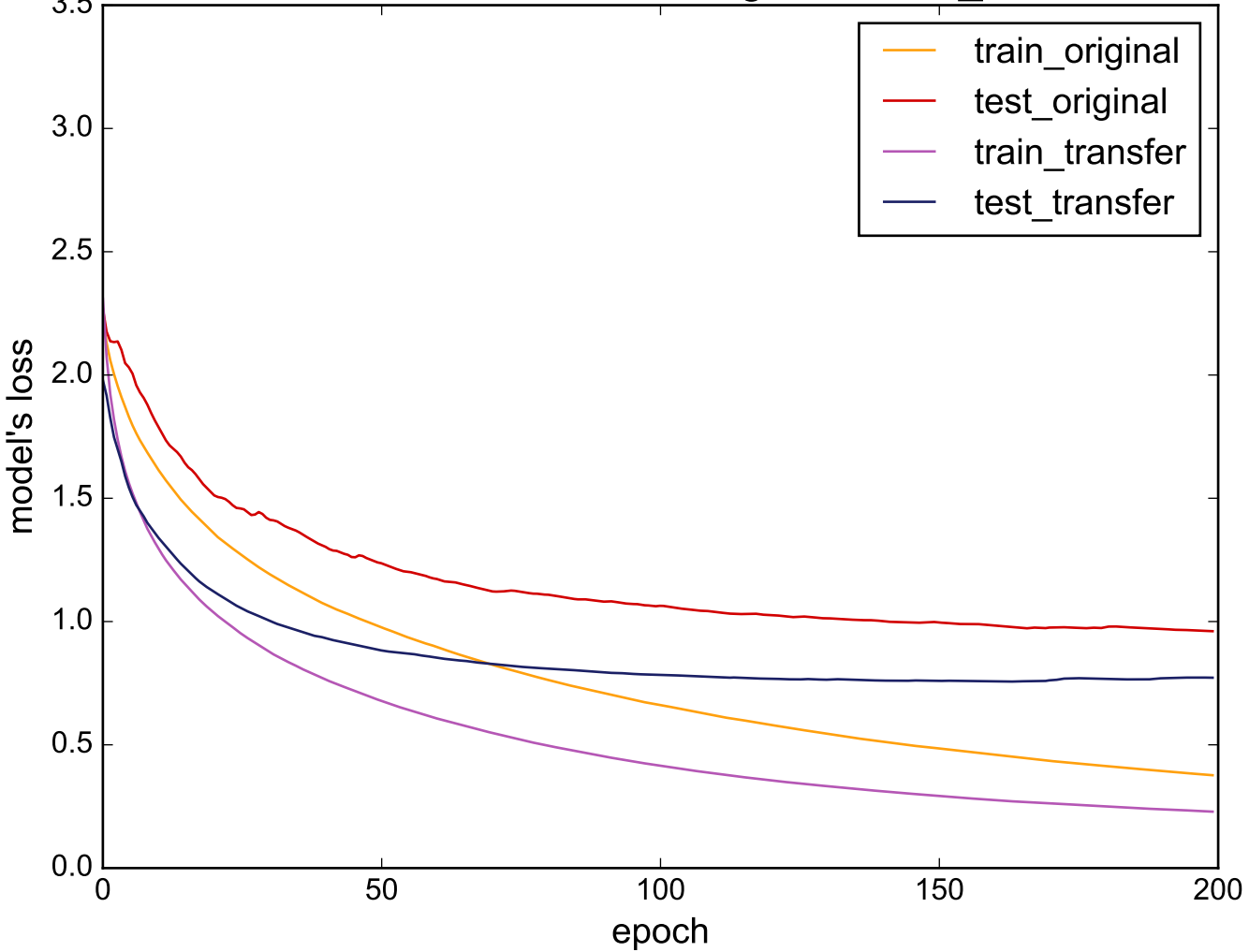
Source: 50words - Target: Cricket_Z
