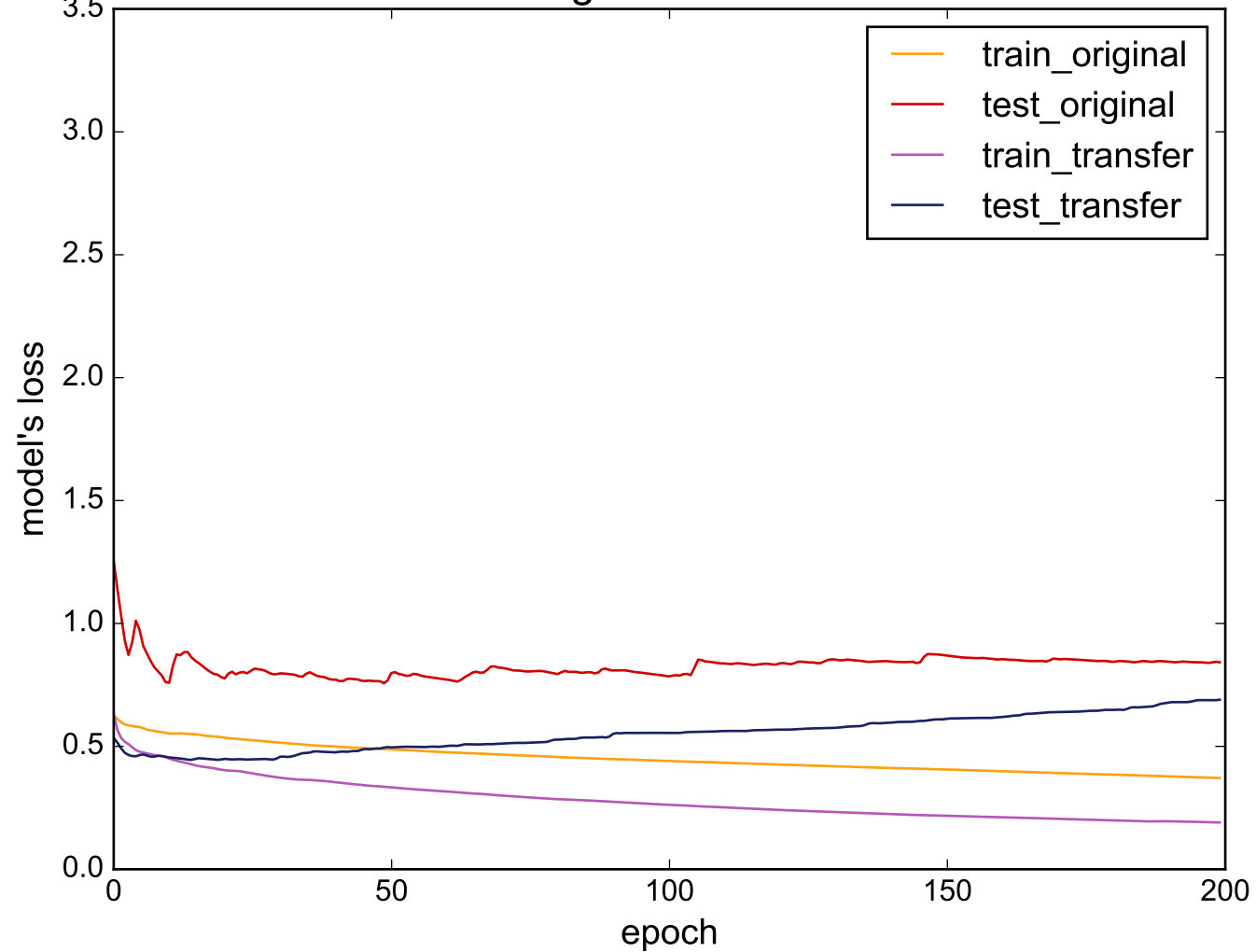
Source: 50words - Target: DistalPhalanxOutlineCorrect
