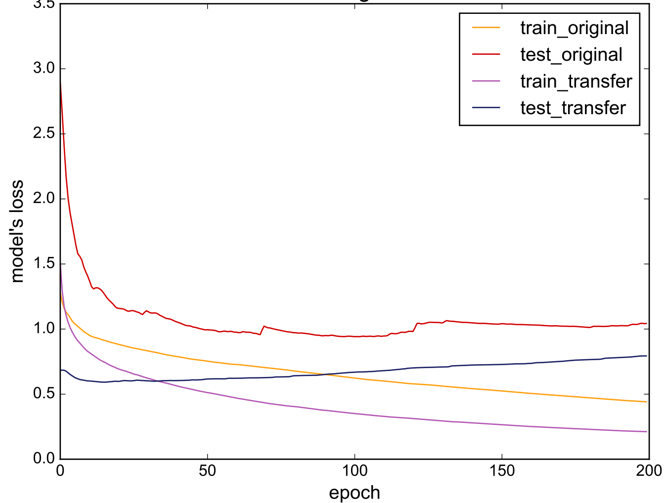
Source: 50words - Target: DistalPhalanxTW
