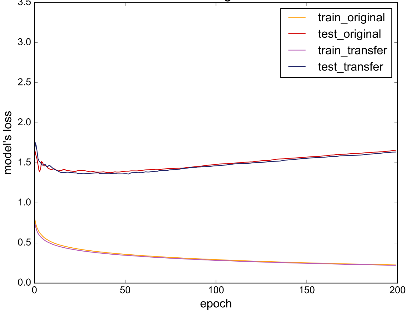
Source: 50words - Target: ElectricDevices
