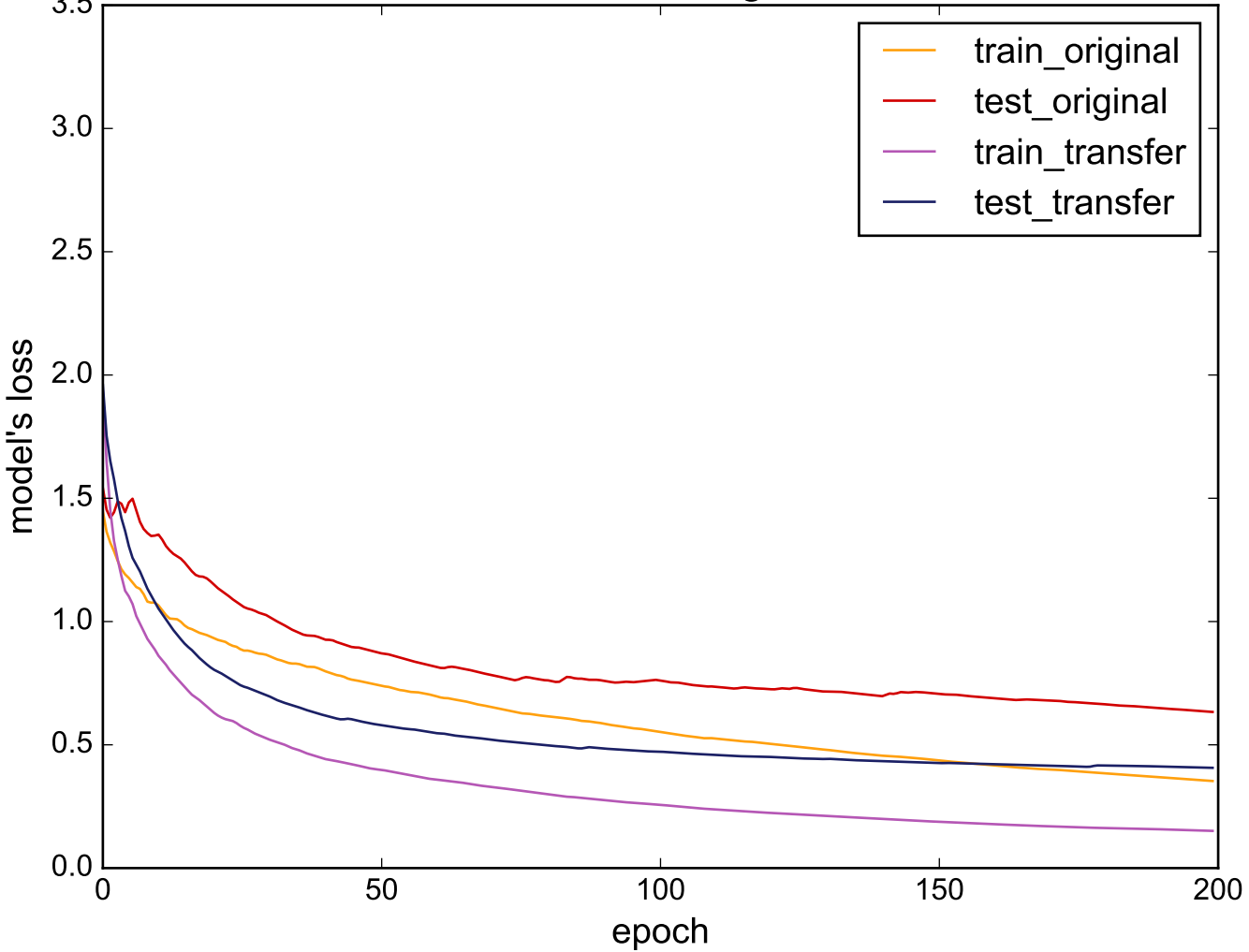
Source: 50words - Target: FaceFour
