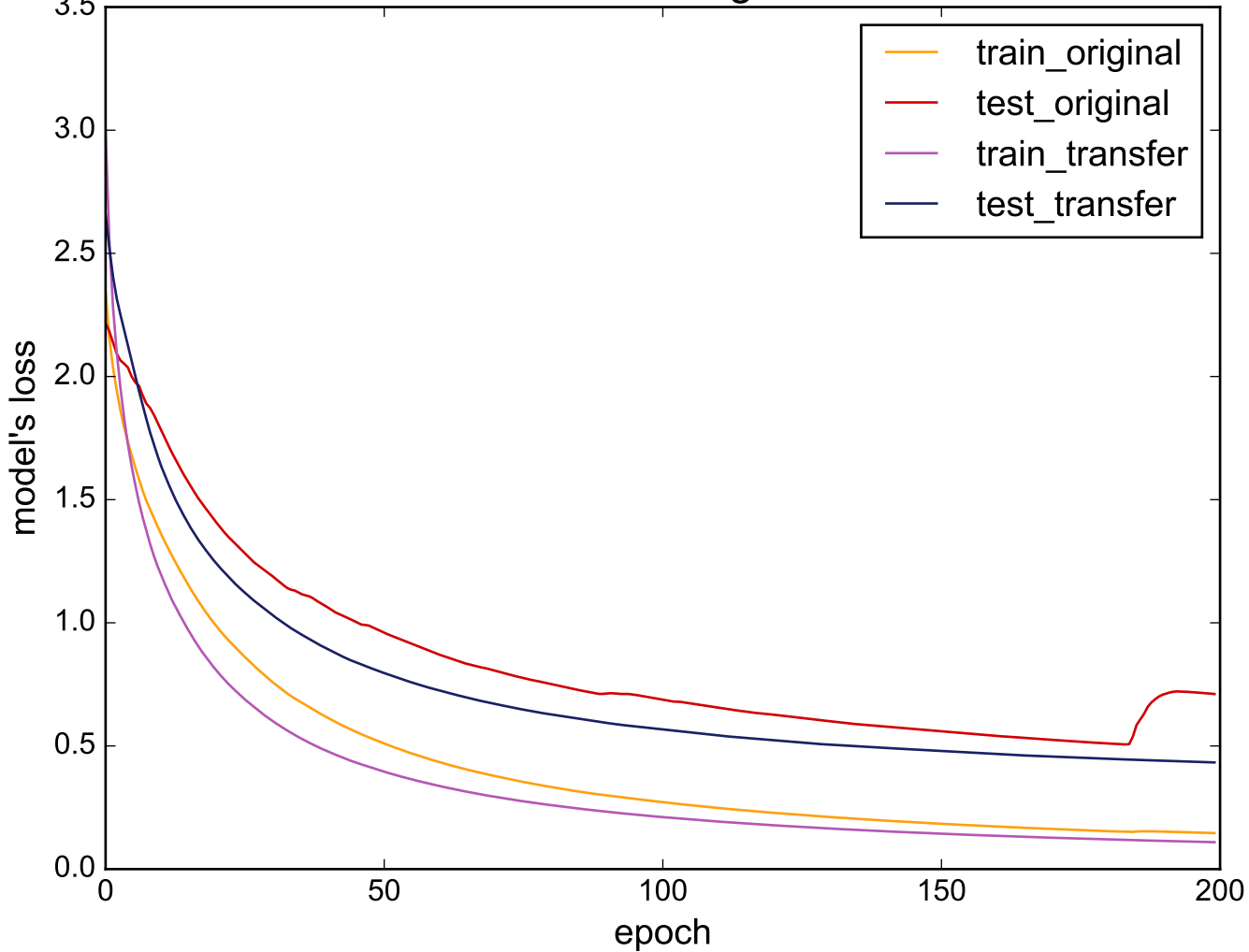
Source: 50words - Target: FacesUCR
