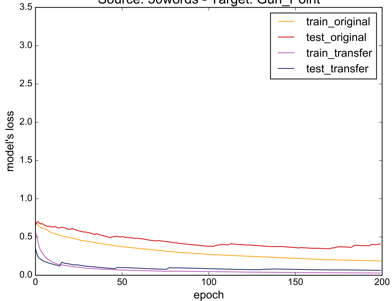
Source: 50words - Target: Gun_Point
