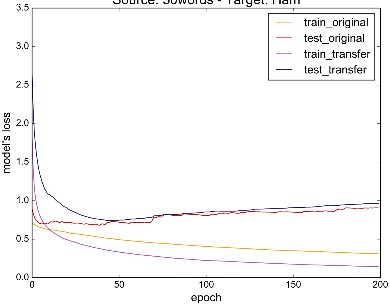
Source: 50words - Target: Ham
