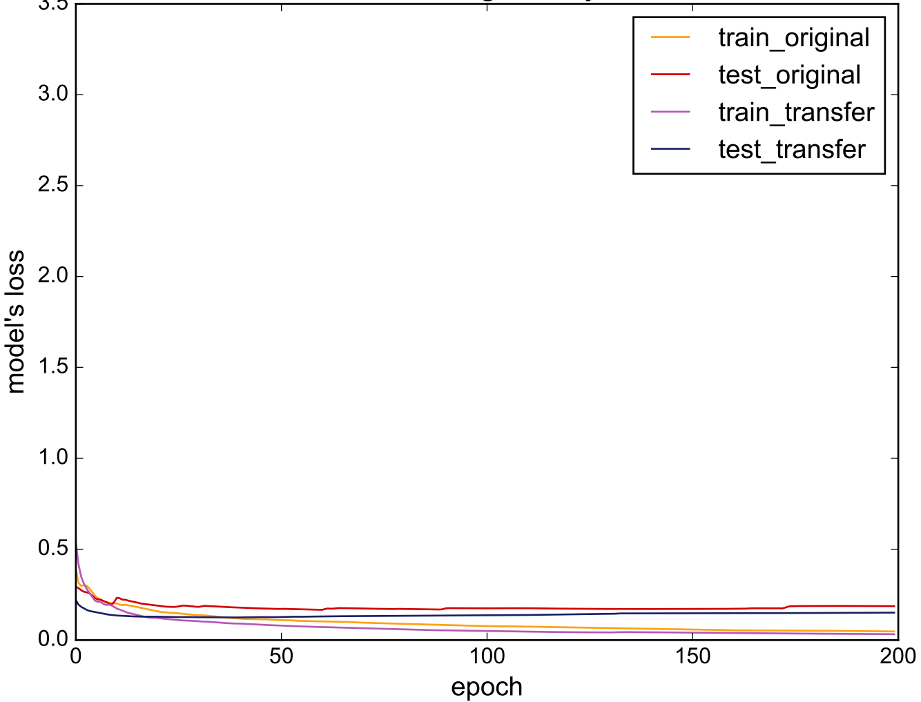
Source: 50words - Target: ItalyPowerDemand
