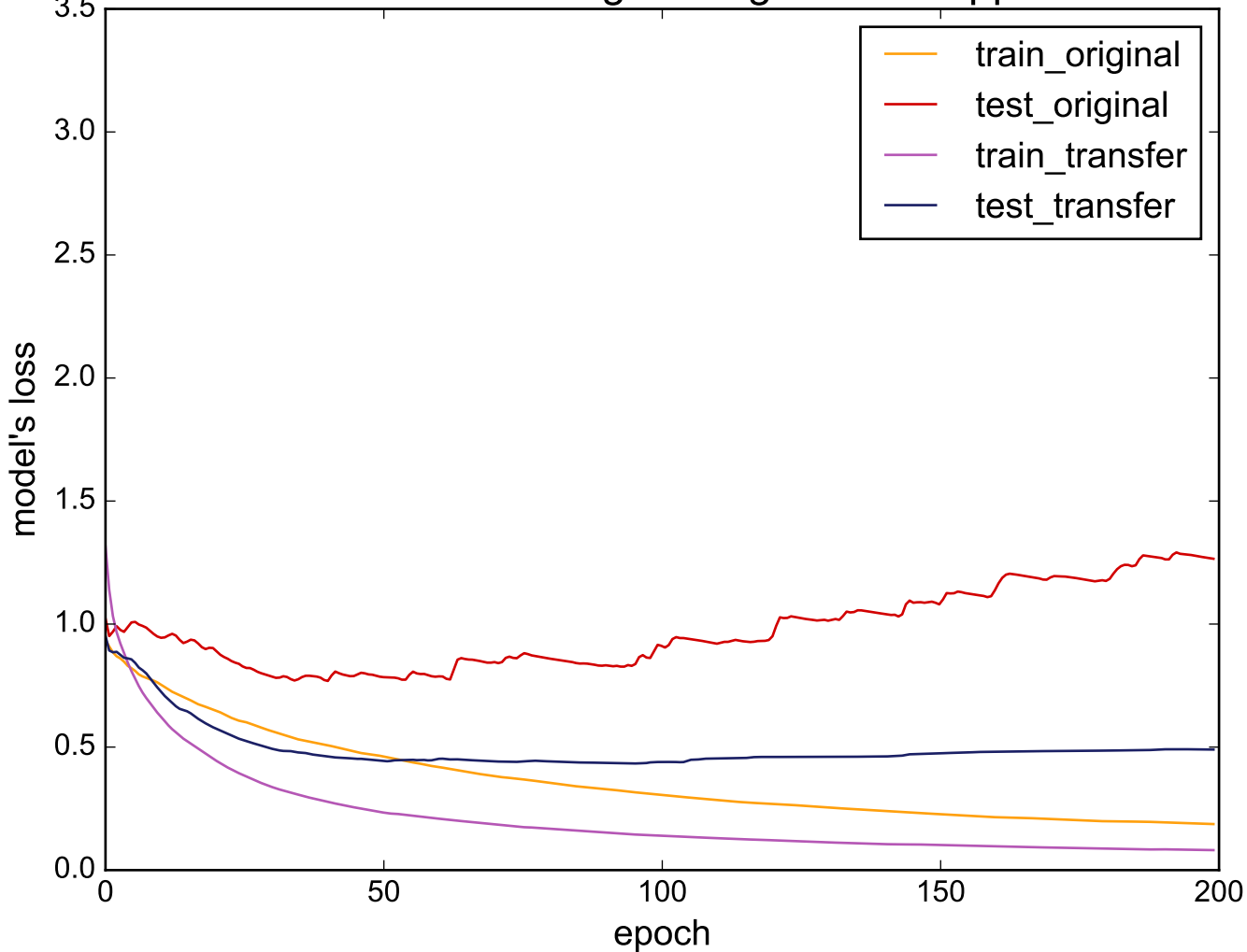
Source: 50words - Target: LargeKitchenAppliances
