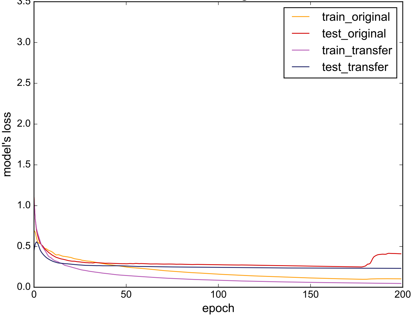
Source: 50words - Target: MoteStrain
