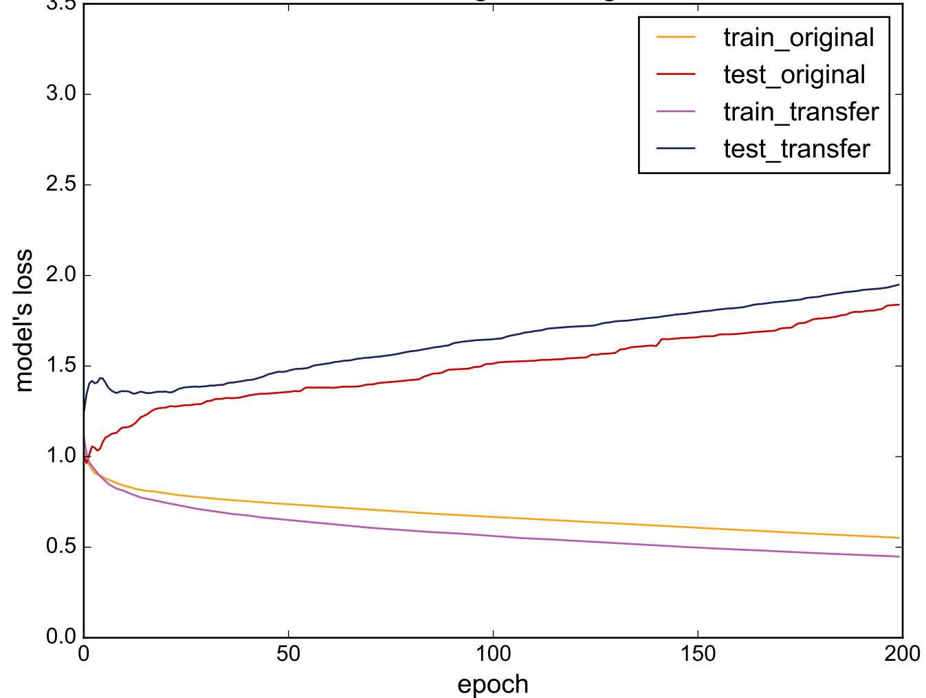
Source: 50words - Target: RefrigerationDevices
