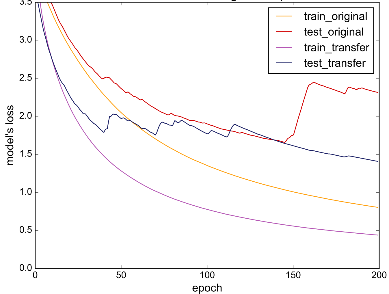
Source: 50words - Target: ShapesAll
