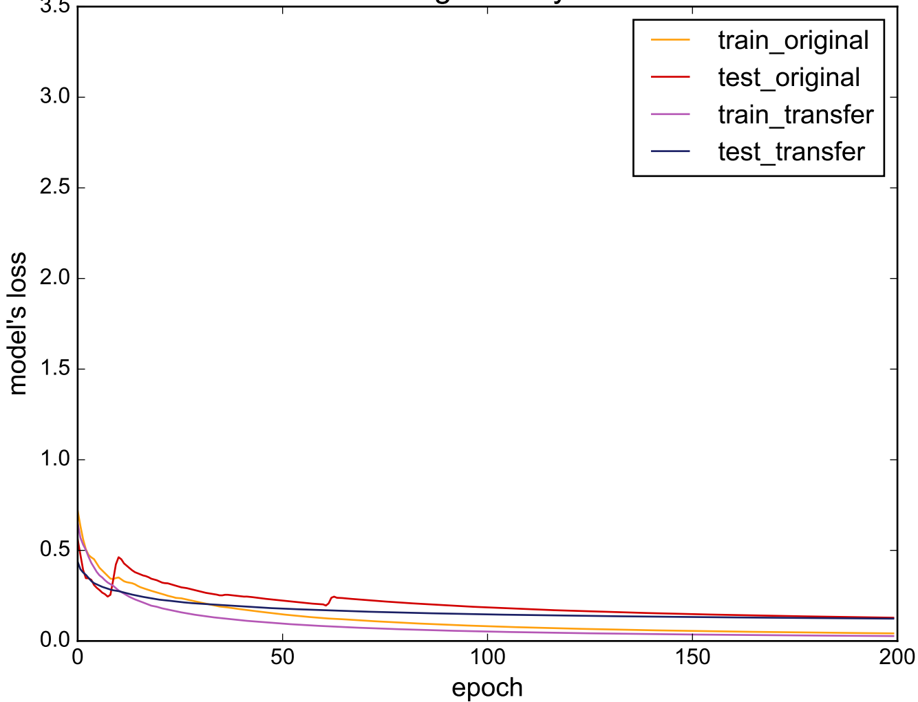
Source: 50words - Target: SonyAIBORobotSurfaceII
