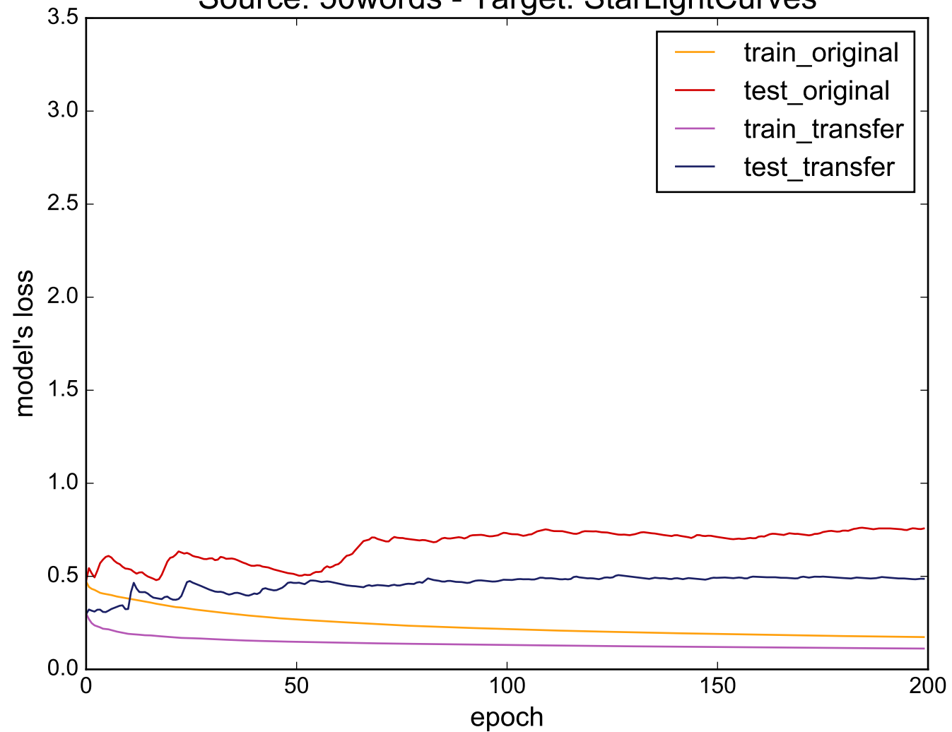
Source: 50words - Target: StarLightCurves
