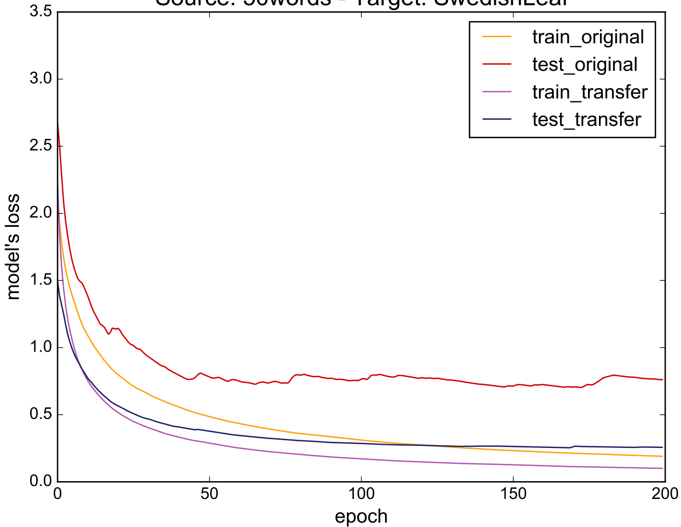
Source: 50words - Target: SwedishLeaf
