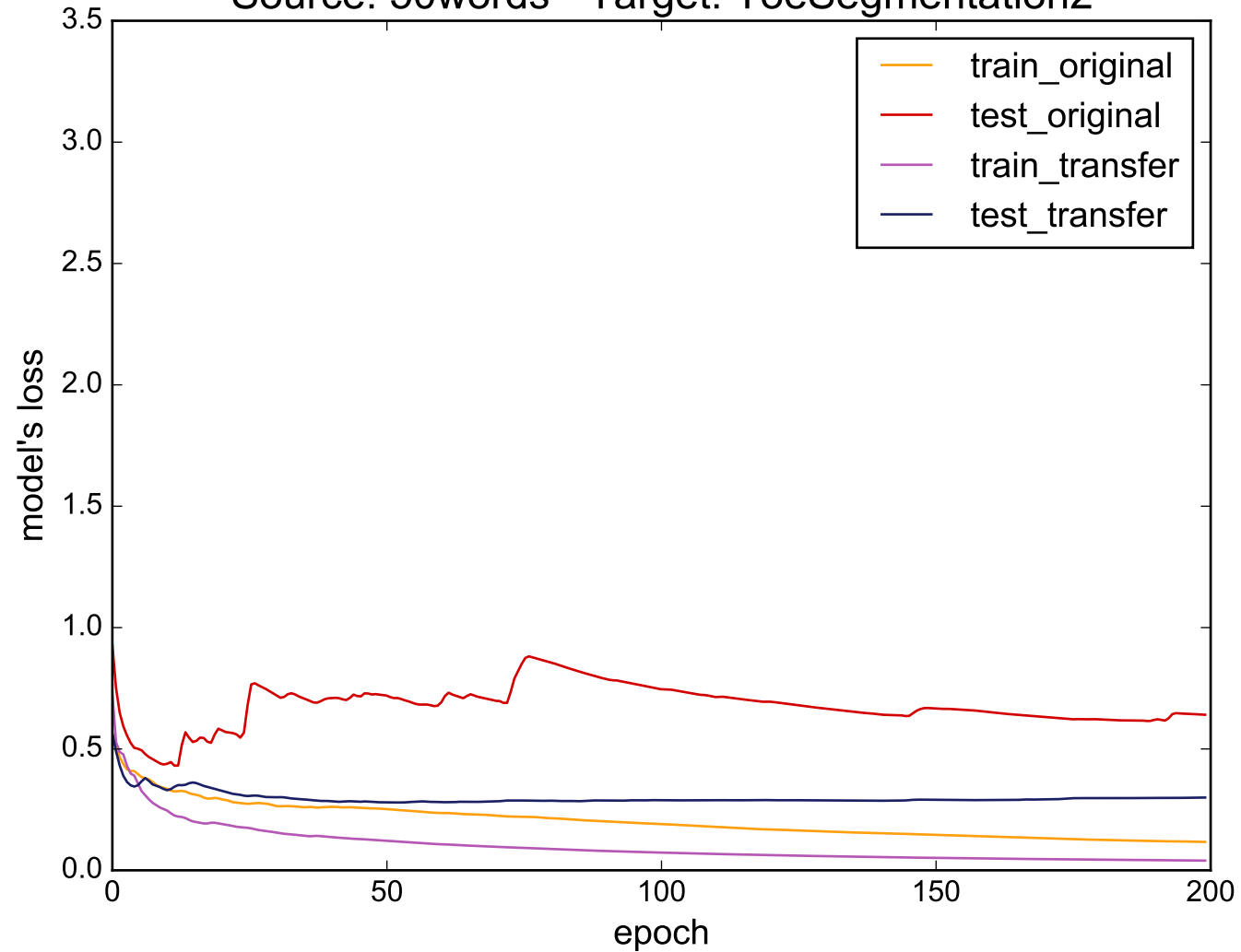
Source: 50words - Target: ToeSegmentation2
