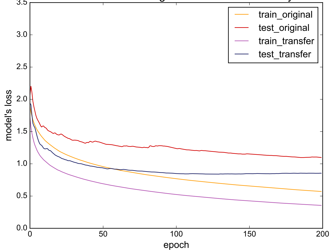
Source: 50words - Target: UWaveGestureLibraryAll
