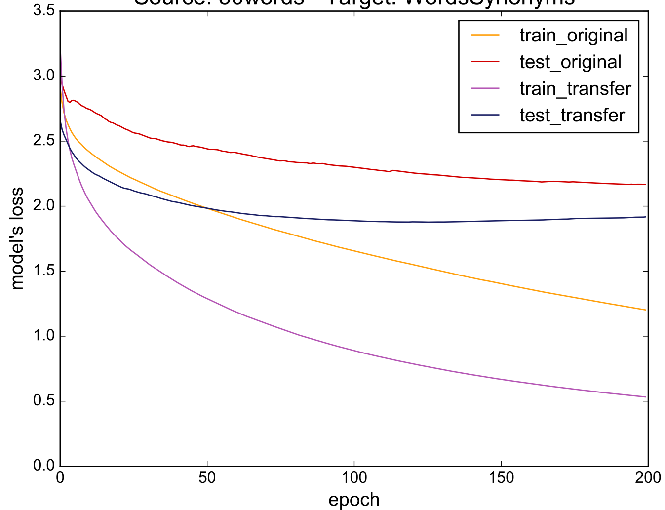
Source: 50words - Target: WordsSynonyms
