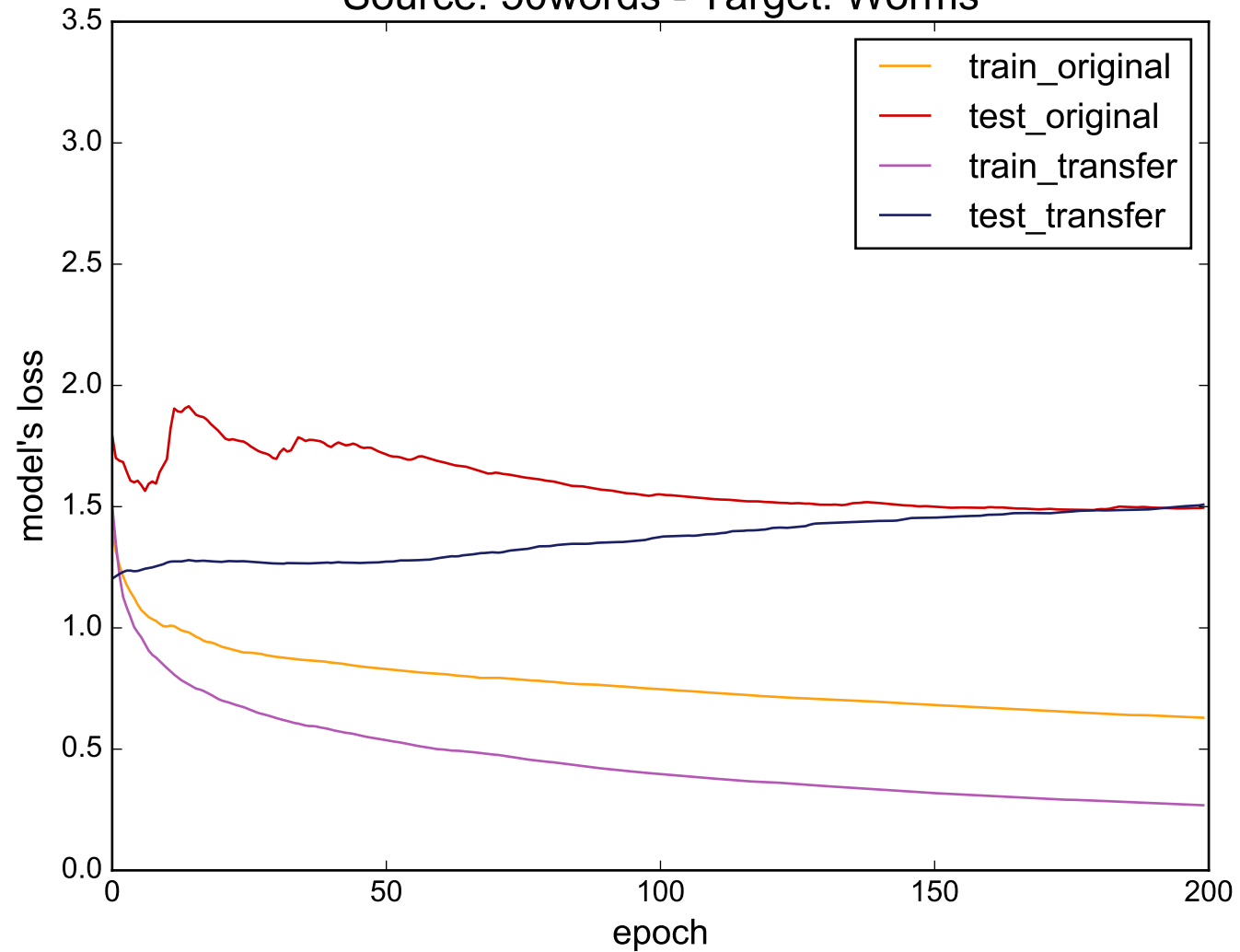
Source: 50words - Target: Worms
