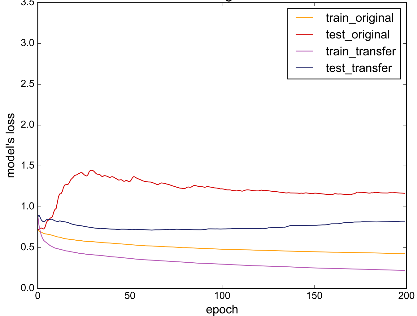
Source: 50words - Target: WormsTwoClass
