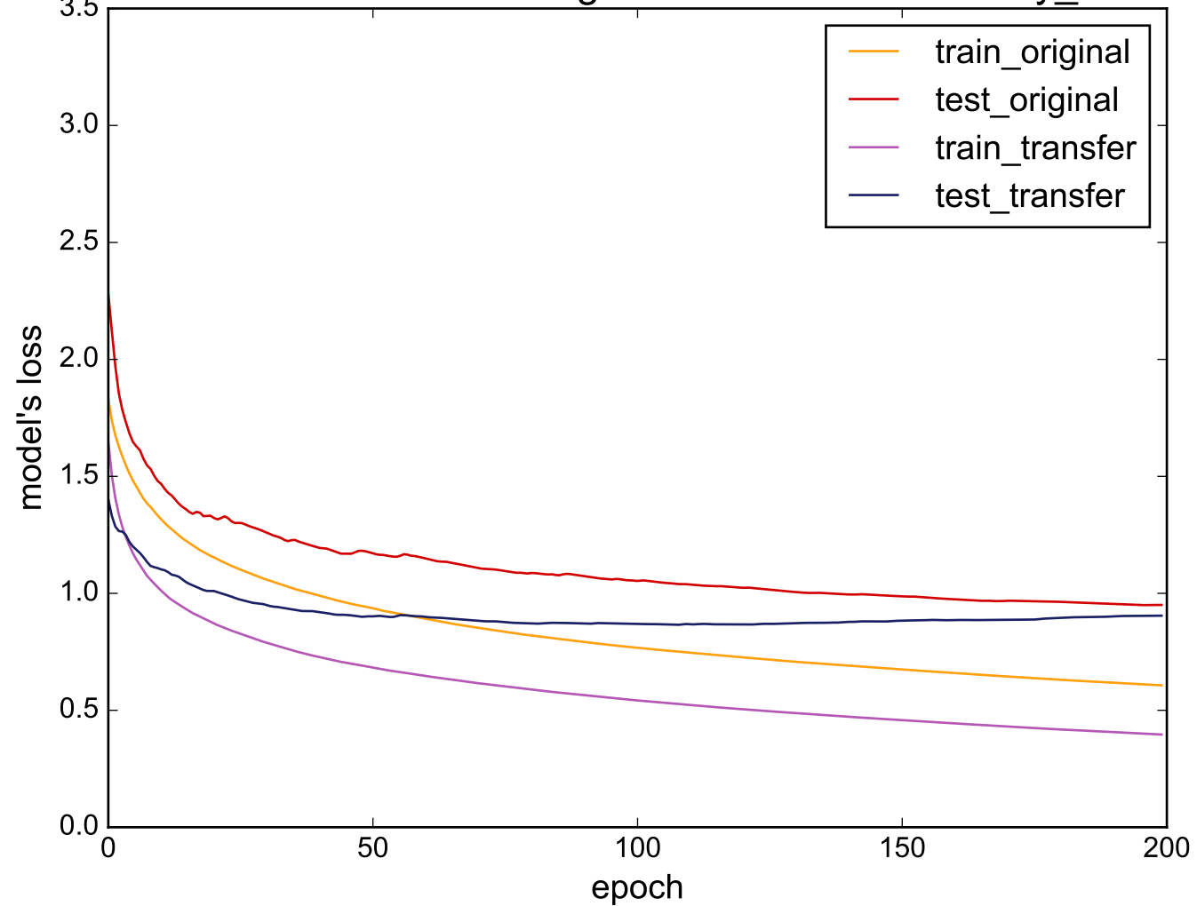
Source: 50words - Target: uWaveGestureLibrary_X
