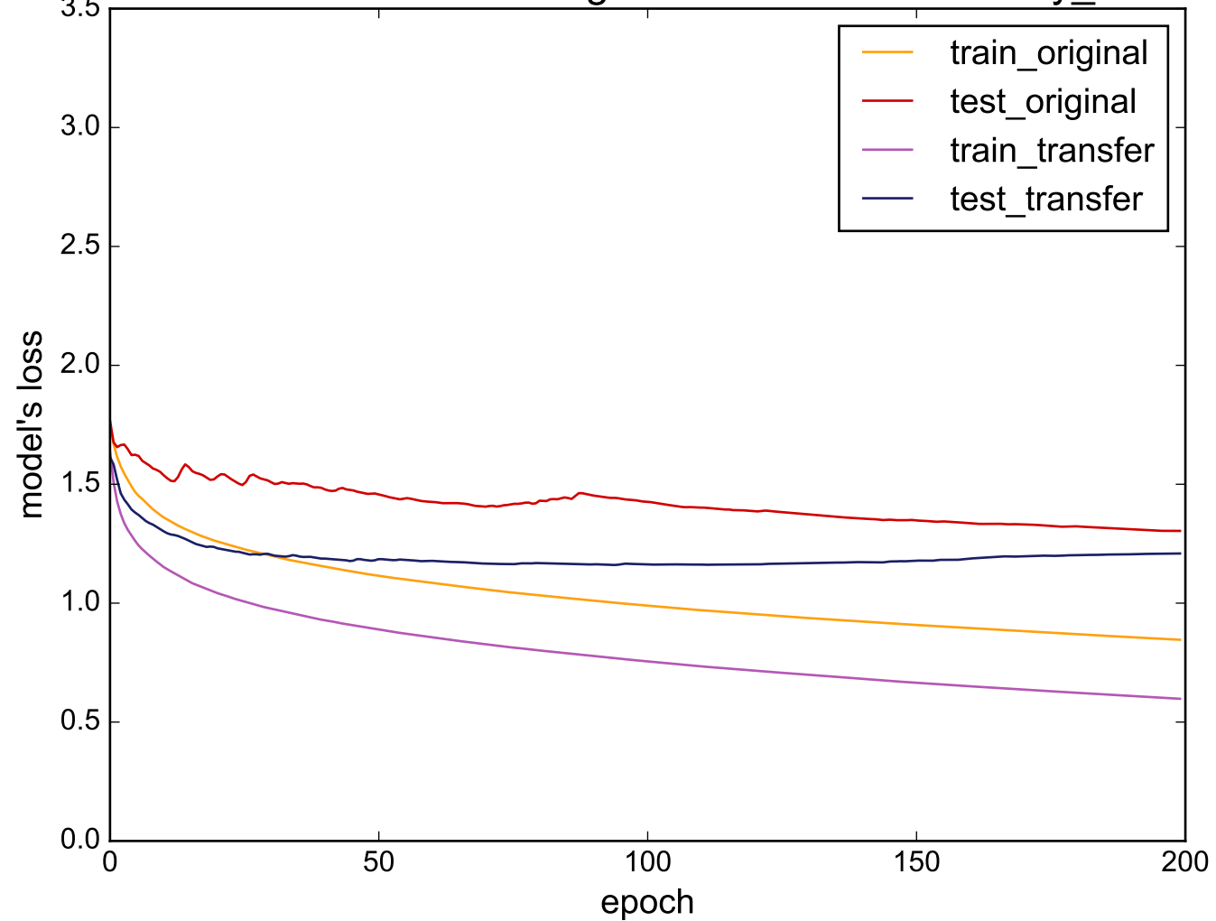
Source: 50words - Target: uWaveGestureLibrary_Y
