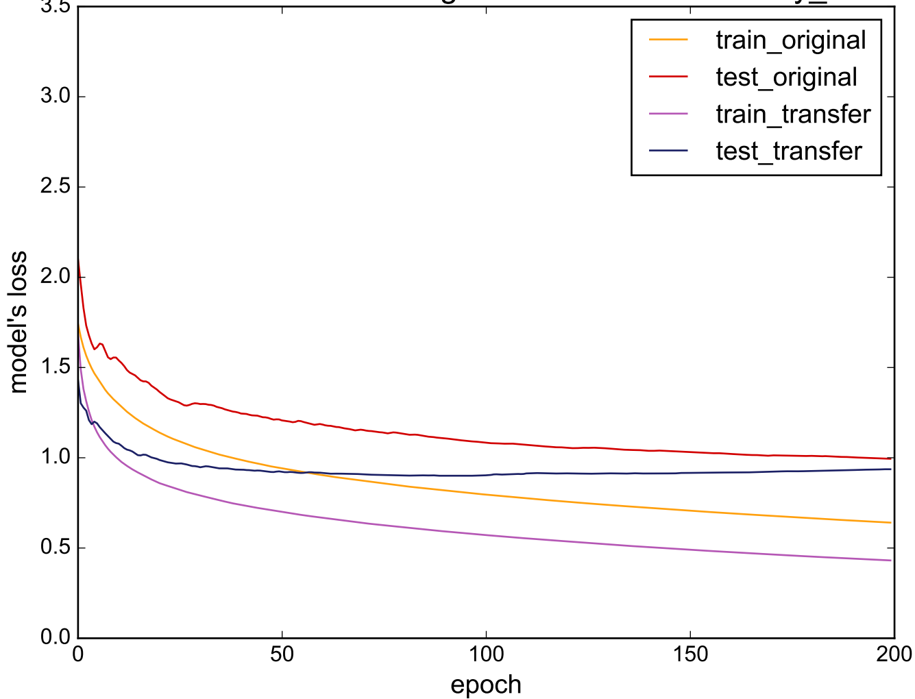
Source: 50words - Target: uWaveGestureLibrary_Z
