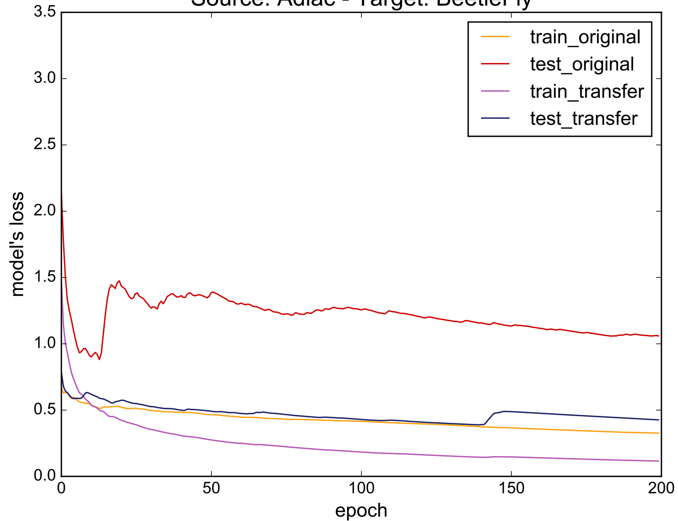
Source: Adiac - Target: BeetleFly
