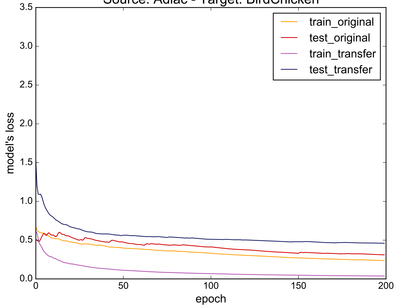
Source: Adiac - Target: BirdChicken
