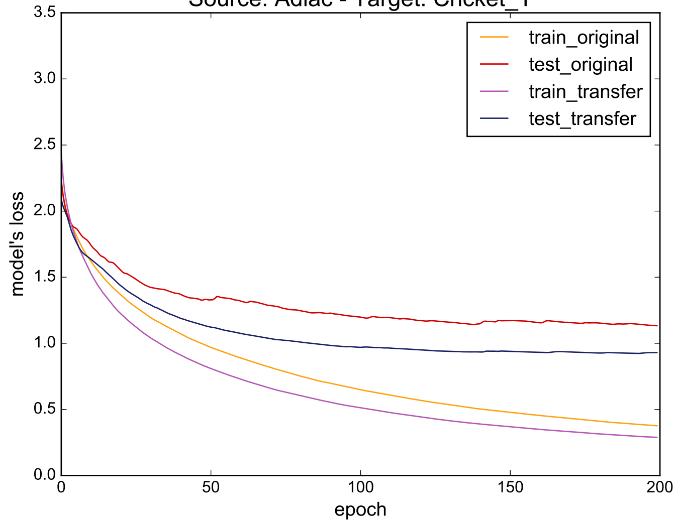
Source: Adiac - Target: Cricket_Y
