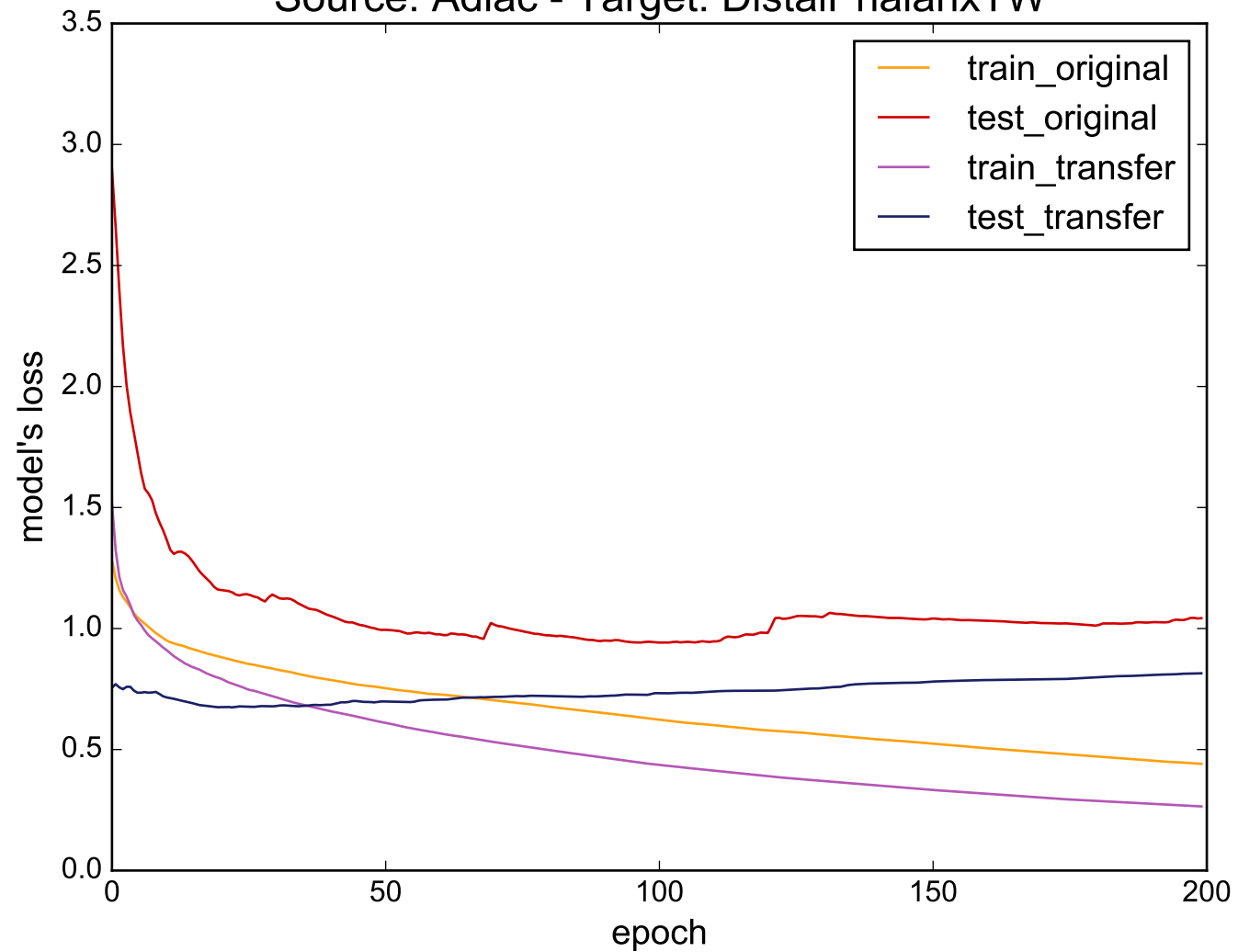
Source: Adiac - Target: DistalPhalanxTW
