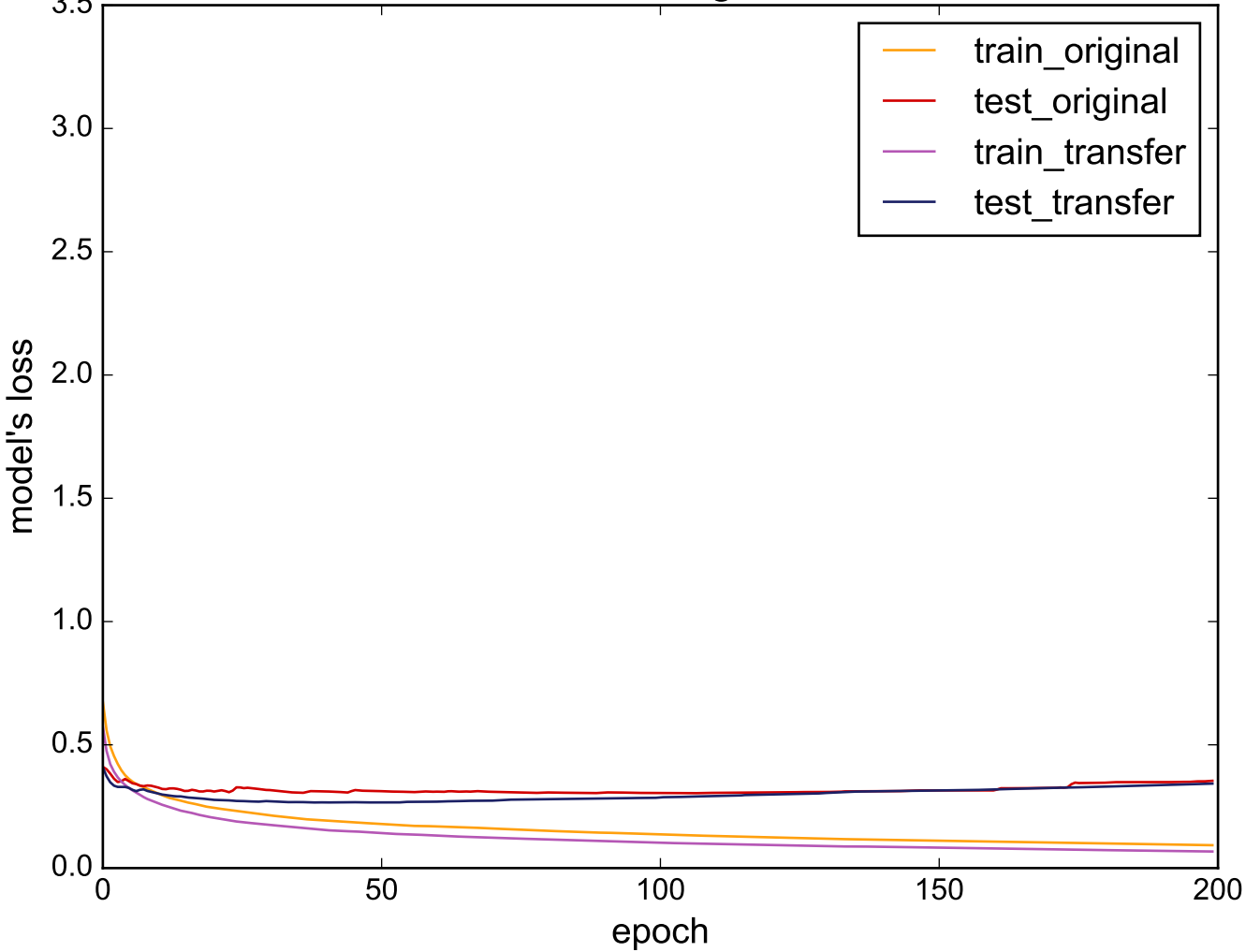
Source: Adiac - Target: ECG5000
