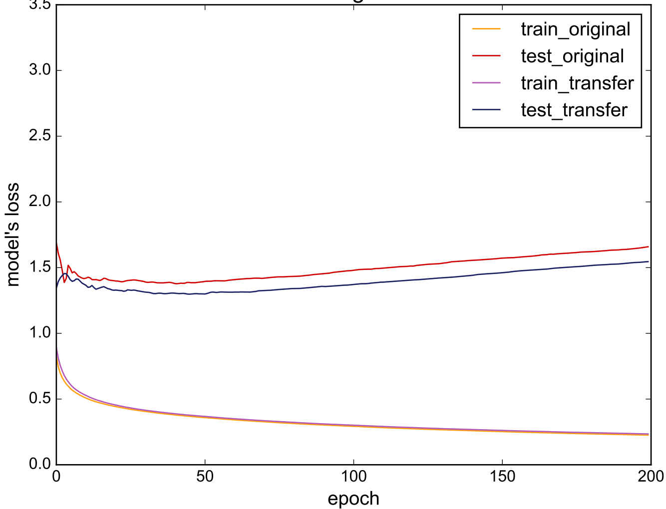
Source: Adiac - Target: ElectricDevices
