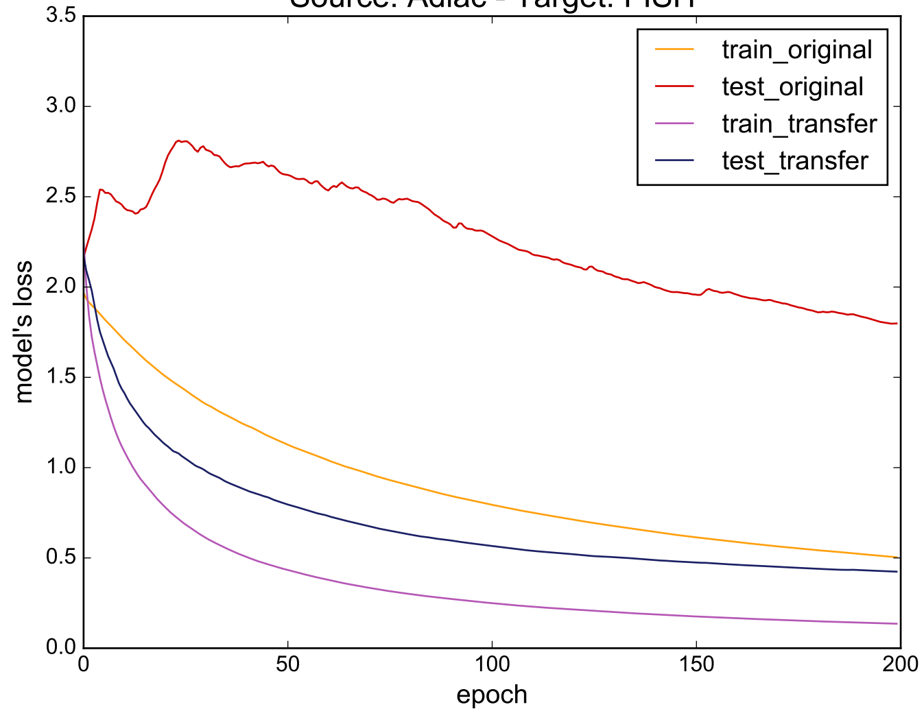
Source: Adiac - Target: FISH
