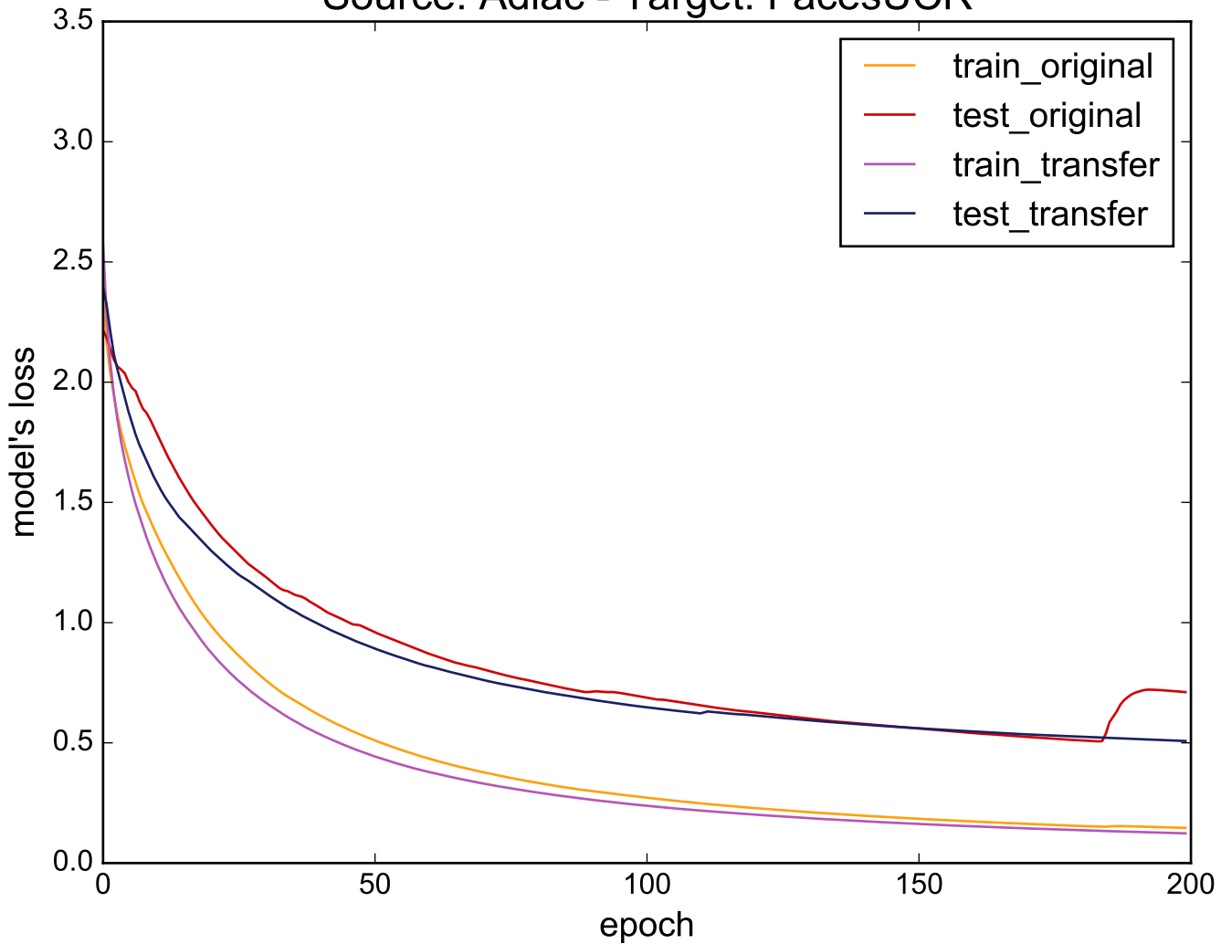
Source: Adiac - Target: FacesUCR
