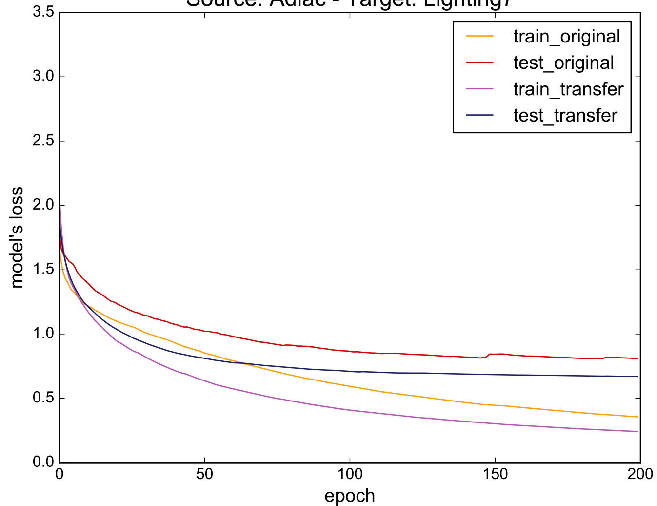
Source: Adiac - Target: Lighting7
