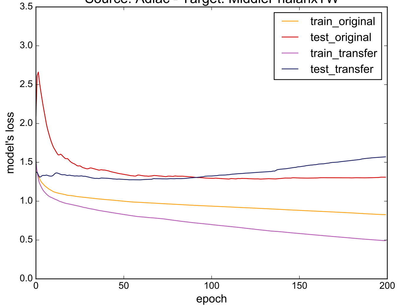
Source: Adiac - Target: MiddlePhalanxTW
