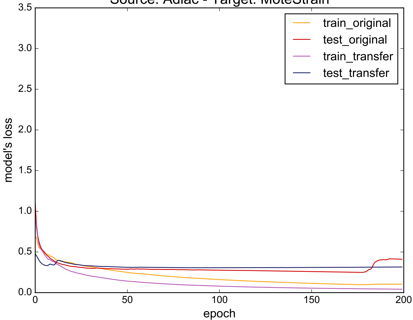
Source: Adiac - Target: MoteStrain
