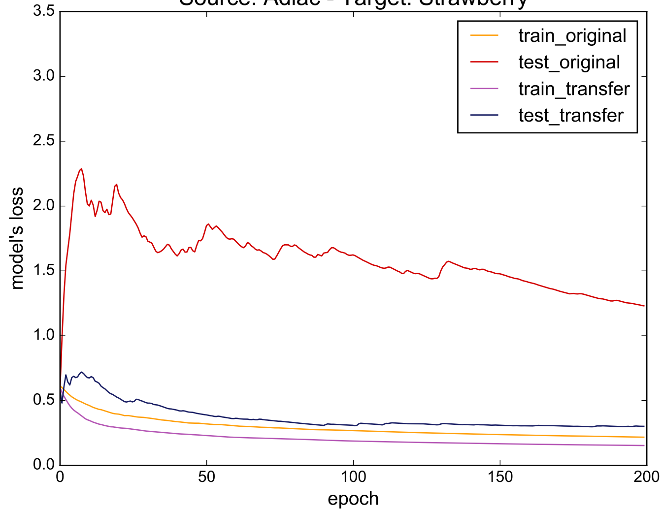
Source: Adiac - Target: Strawberry
