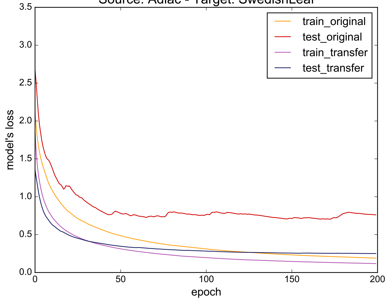
Source: Adiac - Target: SwedishLeaf
