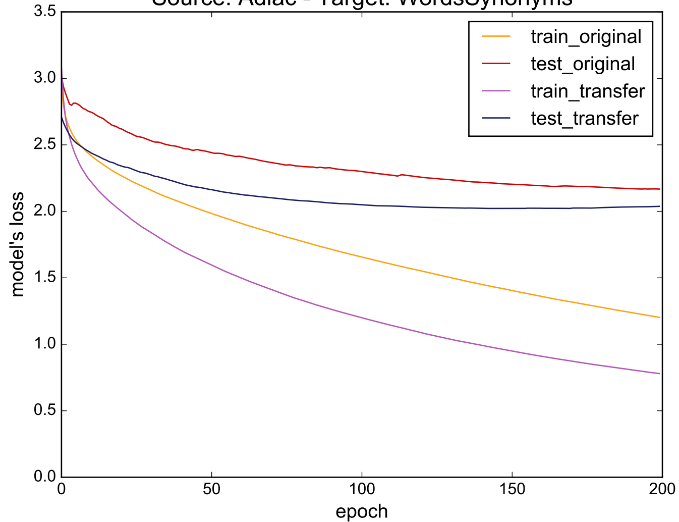
Source: Adiac - Target: WordsSynonyms
