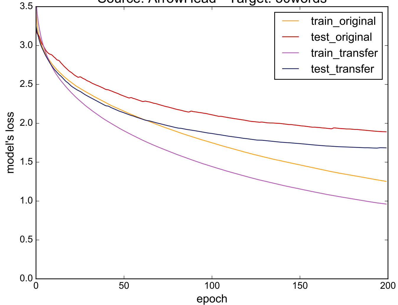
Source: ArrowHead - Target: 50words
