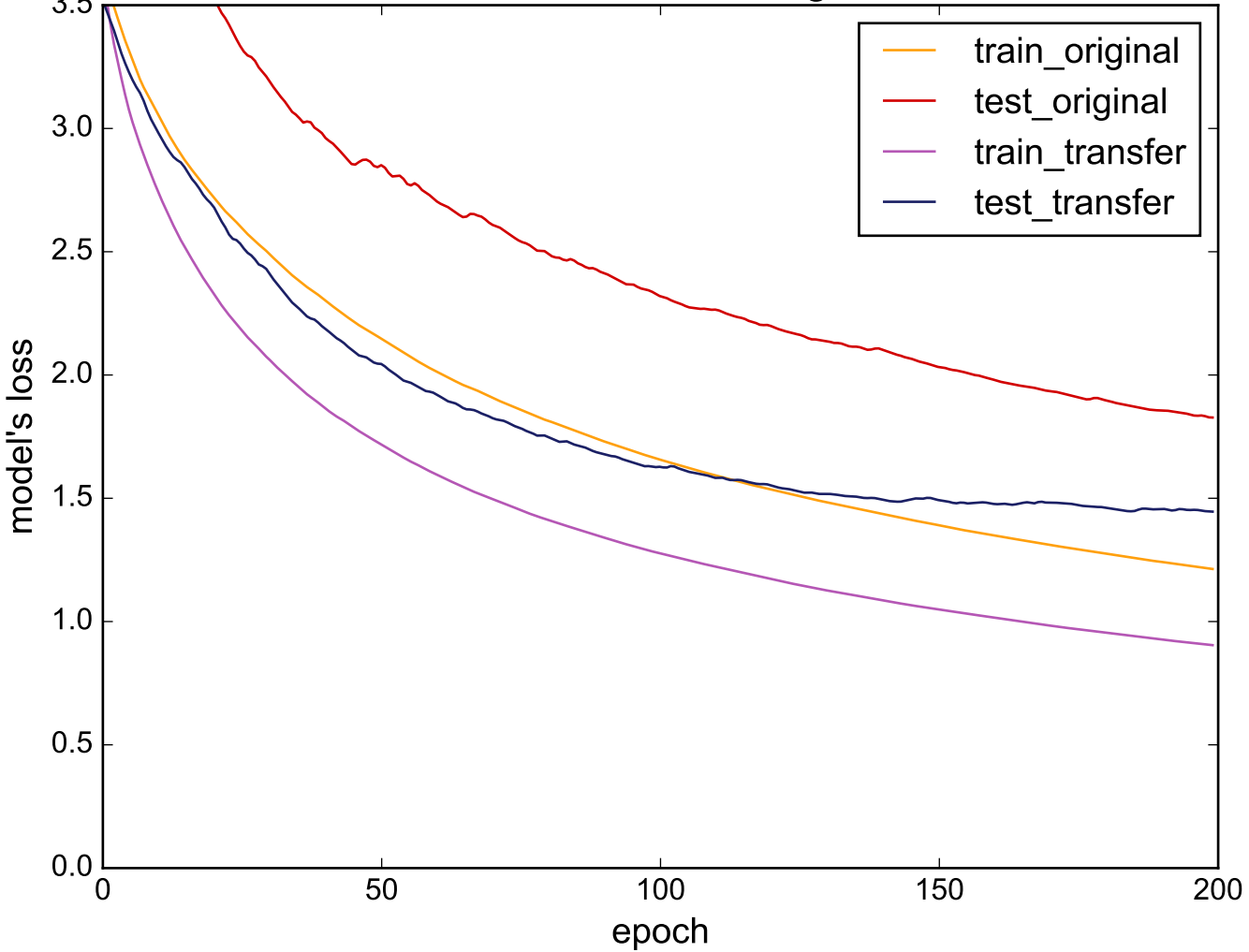
Source: ArrowHead - Target: Adiac
